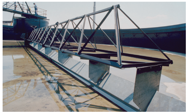
Tow-Bro® Clarifier with unitube hydraulic header for rapid sludge removal.
