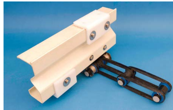
High-strength Loop Chain for heavily loaded tanks and tanks over 200 feet long
