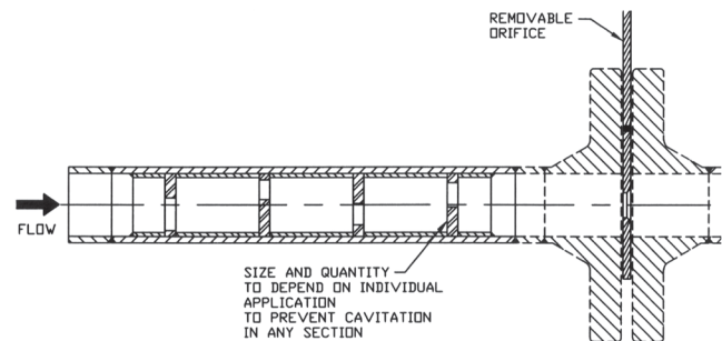
Multi-orifice Assembly
