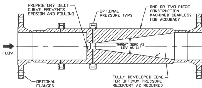
Cavitating Venturi
